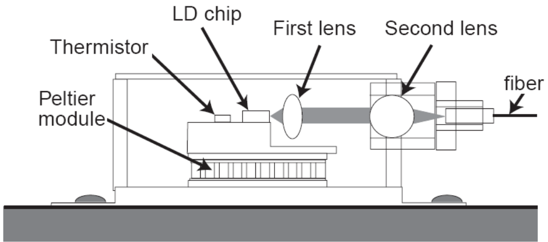
Figure 2 Structure of 1480-nm LD module
