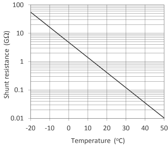
Shunt Resistance - Temperature
