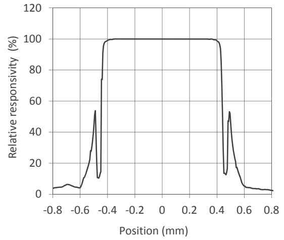
Responsivity Distribution
